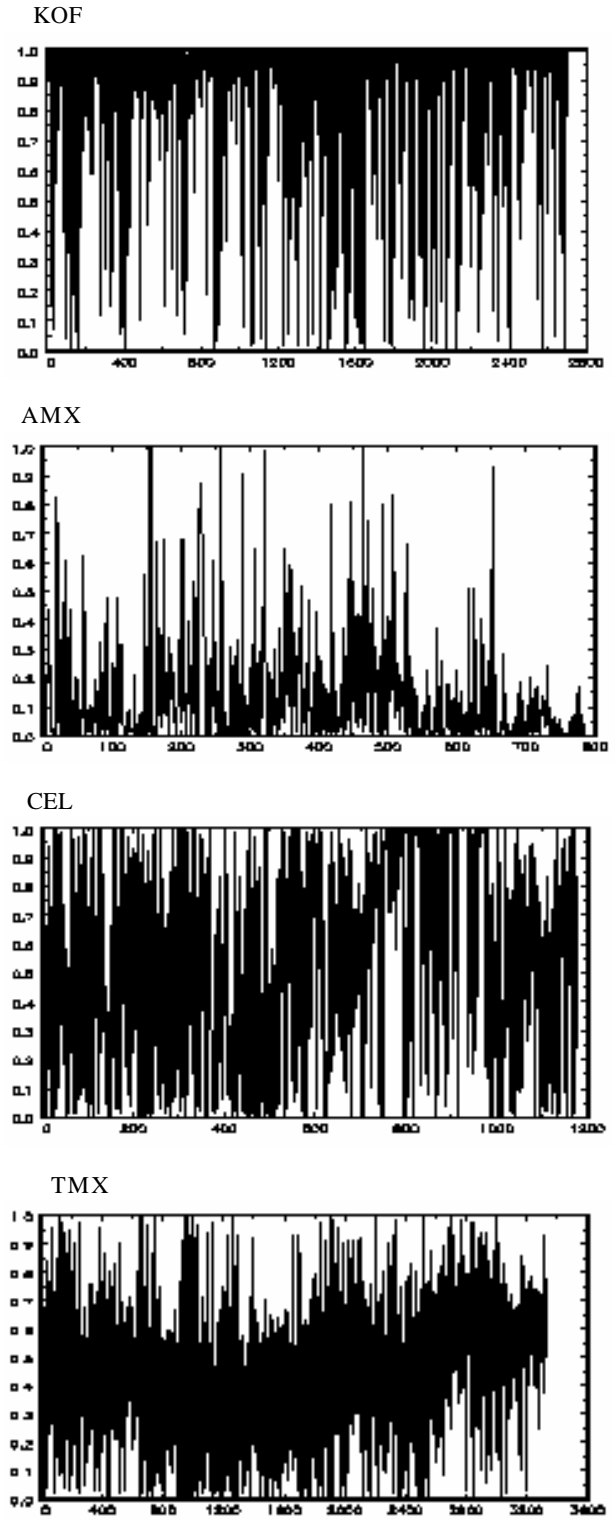
Panel B: Transition Function vs. Time F(Z_{t-d}; \lambda, \mu) v.s. t
