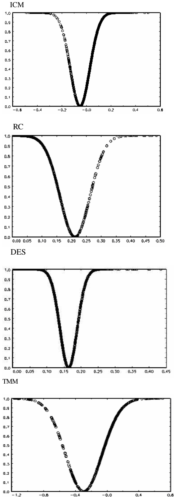
Panel A: Transition Function vs. Transition Variable F(Z_{t-d}; \mathbf{l}, \mu) v.s. Z_{t-d}
