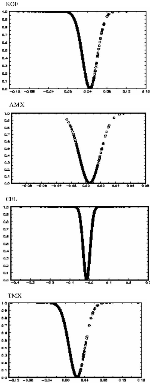
Panel A: Transition Function vs. Transition Variable F(Z_{t-d}; \lambda, \mu) v.s. Z_{t-d}
