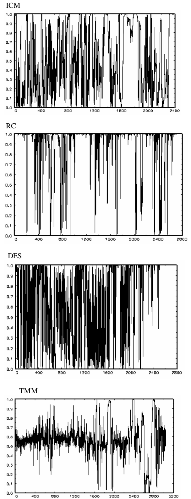
Panel B: Transition Function vs. Time F(Z_{t-d}; \mathbf{l}, \mu) v.s. t
